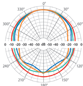
Circular chart of directional characteristic:
