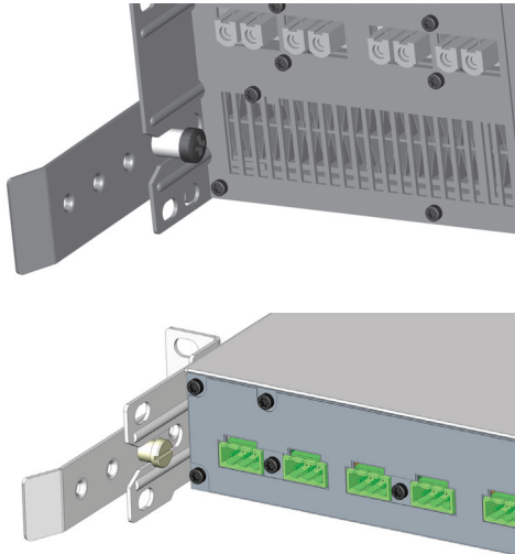
Rear support bracket mounted for removable installation and bracket pointing towards back
