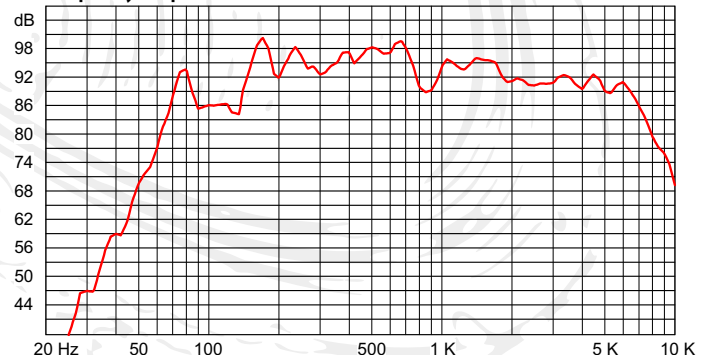
Frequency Response Measured at 2.83v/1m
