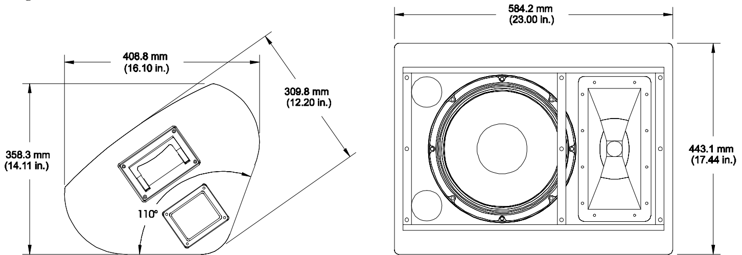
Figure 8—Dimensions
