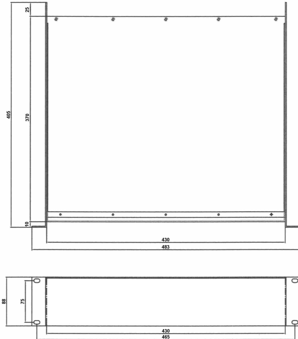
PCL series amplifier dimensions in mm.
